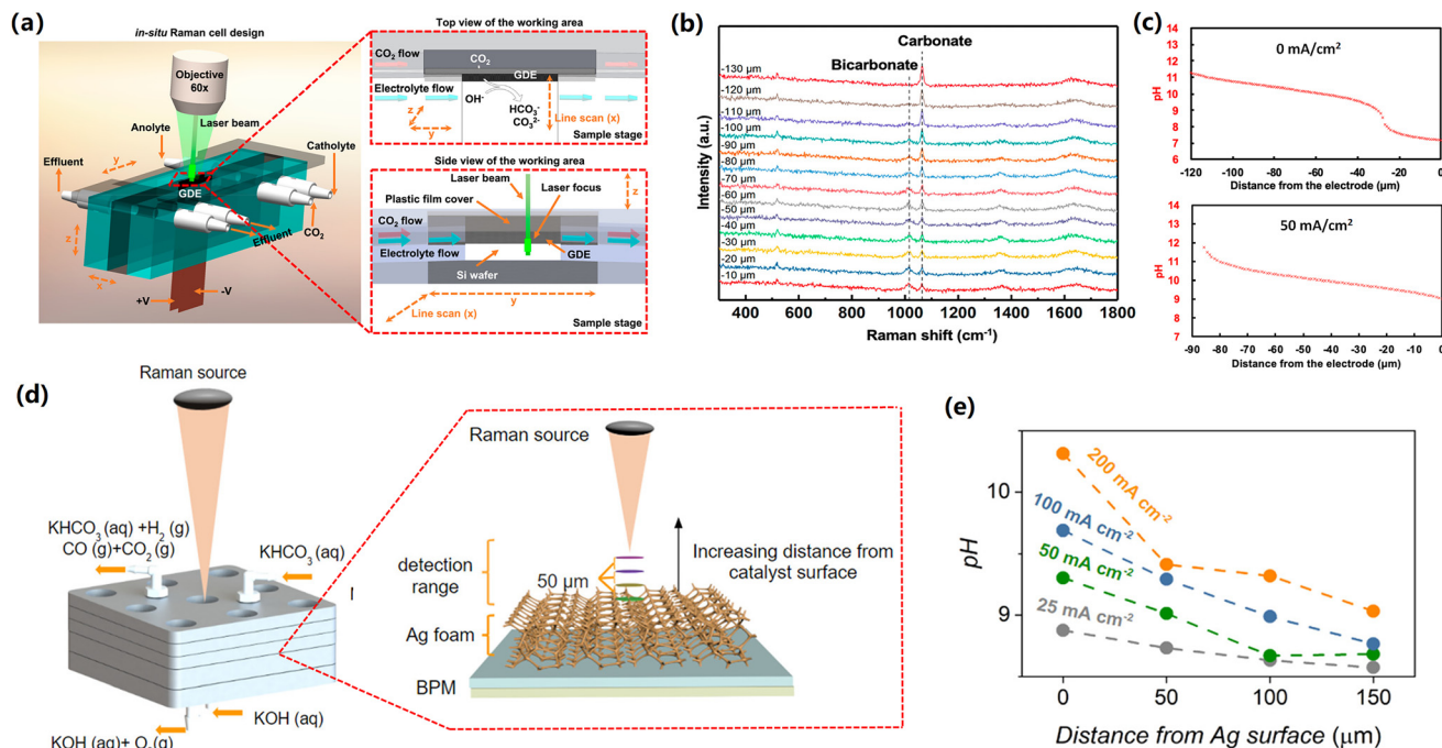
Fig. 5 (a) Schematic illustration of special GDE-type flow cell with top and side views of the cathode area. (b) Raman spectra recorded at various distances from the GDE surface at 0 \text{ mA cm}^{-2} in 1 \text{ M KOH} . (c) pH profile as a function of the distance from the GDE surface in 1 \text{ M KOH} at 0 \text{ mA cm}^{-2} (top) and 50 \text{ mA cm}^{-2} (bottom). These figures have been reproduced from ref. 68 with permission from American Chemical Society, copyright 2020 (d) Schematic illustration of the zero-gap flow cell. Insert shows how different detection planes were measured using the Raman probe. (e) pH profile as a function of the distance from the cathode surface at various current densities in 3 \text{ M KHCO}_3 . These figures have been reproduced from ref. 69 with permission from American Chemical Society, copyright 2020.
