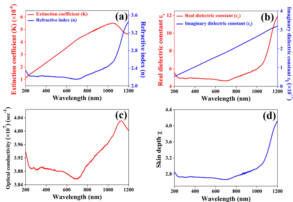
Fig. 9 Plots of (a) extinction coefficient and refractive index, (b) real and imaginary dielectric constants, (c) optical conductivity and (d) skin depth as a function of wavelength for the CuSbSe 2 single crystal.
