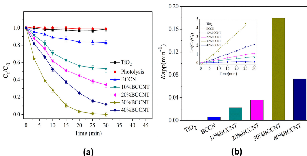
Fig. 23 (a) C_t/C_0 versus time plots of different photocatalysts. (b) Respective kinetic curves (inset) and apparent reaction rate constants of diclofenac (conditions: [DCF]_0 = 10 \text{ mg L}^{-1} , [Catal.] = 1 \text{ g L}^{-1} , no pH adjustment and pH_{\text{initial}} = 5.05 ) and (c) possible mechanism for the photodegradation of DCF and CBZ under LED lamp irradiation over 30% BCCNT composites. Reproduced from ref. 719 with permission from Elsevier (2019).
