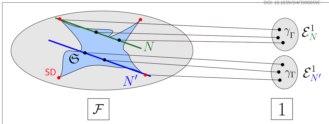
Figure 3. Illustration of the one-to-one relation between the set \mathcal{S} (light blue) of free states on the Fock space \mathcal{F} (gray) and the sets of 1RDMs \mathcal{E}_N^1 for two different particle numbers N, N' . The red dots illustrate its extremal elements which are the Slater determinants. For fixed particle number N , the free states \Gamma corresponding to 1RDMs \gamma_\Gamma \in \mathcal{E}_N^1 lie on a hyperplane with average particle number \langle \hat{N} \rangle_\Gamma = N .
