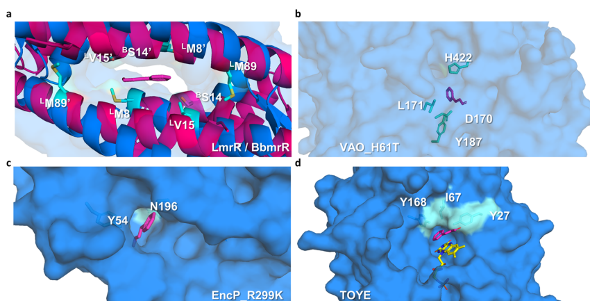
Fig. 2 Selection of residues for mutagenesis. (a) For BbmrR (pink ribbon), analysis was carried out by comparing it with LmrR (blue ribbon), as a previously described active scaffold. Positions S14 of BbmrR are highlighted along with the residues chosen for LmrR, labelled with B or L, respectively. (b–d) Substrate-guided scaffold surfaces of (b) VAO_H61T, (c) EncP_R299K, and (d) TOYE are shown in light blue. The transparency settings for VAO_H61T are adjusted to highlight the inner residues. The substrate is shown in pink (PDB 9Y6), and selected residues are highlighted in cyan. Modeling was performed using the program AutoDock ( https://vina.scripps.edu/ ).
