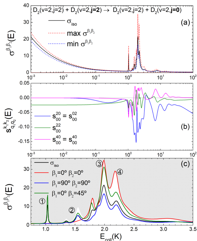
Fig. 7 (a) Isotropic cross section (solid black curve) as a function of E_{\text{coll}} for \text{D}_2(v = 2, j = 2) + \text{D}_2(v = 2, j = 2) \rightarrow \text{D}_2(v = 2, j = 2) + \text{D}_2(v = 2, j = 0) collisions. The maximum and minimum values of the cross sections that could be achieved by a given alignment of the two internuclear axes of the diatoms are shown as red and blue dashed curves, respectively. (b) The relevant polarization parameters, s_{q_1 q_2}^{k_1 k_2} , are shown as a function of E_{\text{coll}} . (c) \sigma^{\beta_1 \beta_2} calculated as a function of E_{\text{coll}} for three given preparations. The region above the maximum value of the cross section that could be achieved is shaded in grey. The labels 1–4 indicate the E_{\text{coll}} at which the dependence on \sigma^{\beta_1 \beta_2} is displayed in Fig. 9.
