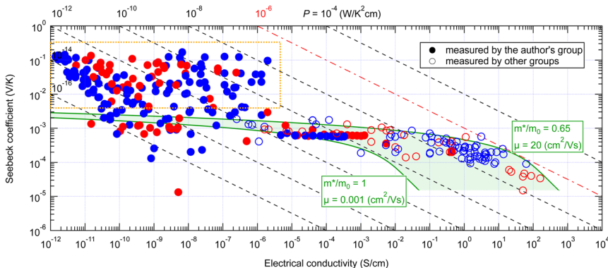
Fig. 3 Seebeck coefficient and electrical conductivity of various organic small-molecule semiconductors in the temperature range near 300–360 K. The green shaded area indicates the possible range of the values calculated from eqn (2) and (3). Red marks indicate positive Seebeck coefficients and blue ones negative. Filled marks are measured by the authors' group and transparent ones by other groups. The orange box indicates the area of the giant Seebeck effect. A table of values and reference information is available as ESI.†
