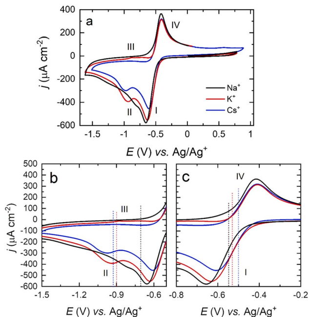
Fig. 5 (a) Cyclic voltammograms of a Pt(poly) electrode in an O_2 -saturated DMSO solution containing 0.1 M NaClO_4 (black), KClO_4 (red) and CsClO_4 (blue), at 50 \text{ mV s}^{-1} scan rate. Expanded view of the potential range corresponding to the formation of O_2^{2-} (b) and O_2^- (c). Dotted lines represent the E_{1/2} of the ORR half reactions for Na^+ (black), K^+ (red) and Cs^+ (blue).
