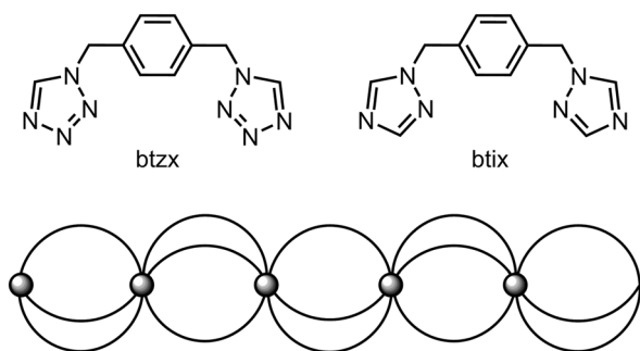
Scheme 6 The ditopic bis-(azoly)methylbenzene ligands employed in ref. 144–146, and a schematic of their 1D iron(II) coordination polymers.
