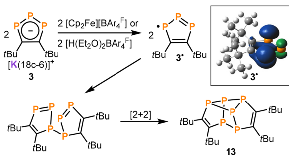
Scheme 4 Proposed mechanism for the formation of 13 by oxidation of 3 ; the inset shows the calculated spin density distribution of 3* drawn at a surface isovalue at 0.05.
