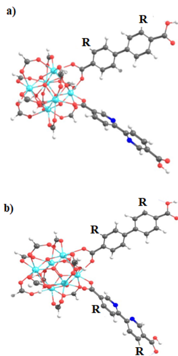
Fig. 2 Schematic representation of the finite structure (Zr-node/linkers) with the substituents R ( -H , -NH_2 , and -SH ) in (a) the bpdc ( 1A-bpdc-R ) and (b) both linkers ( 1A-R ). Atoms are denoted with dark gray (carbon), light gray (hydrogen), red (oxygen), darker blue (nitrogen), and blue (zirconium).
