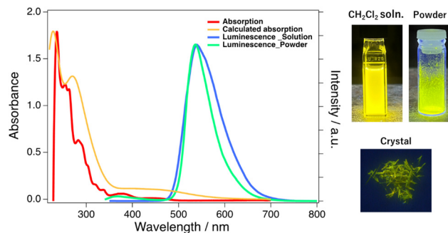
Fig. 3 (a) Absorption spectrum of R -Zn (red, 1.0 \times 10^{-5} M in CH 2 Cl 2 ), the calculated spectrum (orange), and emission spectra in 1.0 \times 10^{-4} M CH 2 Cl 2 solution (blue) and in powder (green) excited at 300 nm; (b) photographs of emission of R -Zn in a CH 2 Cl 2 solution (upper left), in powder (upper right) and in crystals (lower).
