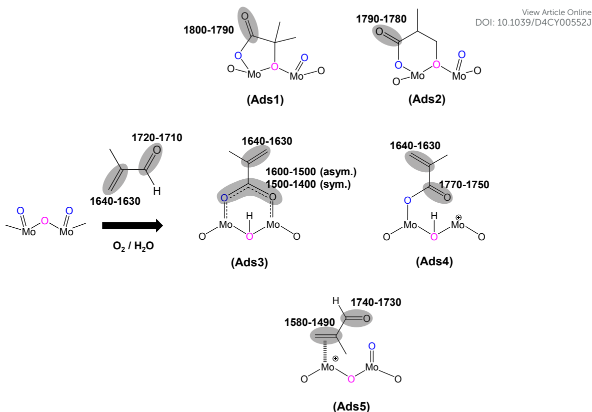
Figure 3 Proposed surface species under MAL reaction conditions at 320 °C over HPA catalysts: 5-membered ring lactone-type species ( Ads1 ), 6-membered ring lactone-type species ( Ads2 ), bidentate methacrylate species ( Ads3 ), monodentate methacrylate species ( Ads4 ), and \pi -adsorbed species [ Ads5 ].
