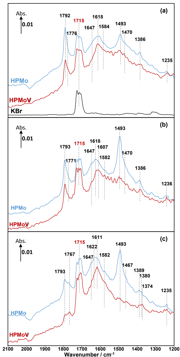
Figure 2 Comparison of in-situ DRIFT spectra recorded at 320 °C over \text{H}_3\text{PMoO}_{12}\text{O}_{40} and \text{H}_4\text{PMoO}_{11}\text{VO}_{40} at 2 min under MAL (a), MAL+ \text{O}_2 (b), and MAL+ \text{O}_2 + \text{H}_2\text{O} (c). Gas feed is composed of 3500 ppm MAL (when added), 7000 ppm \text{O}_2 (when added), 7000 ppm \text{H}_2\text{O} (when added), and Ar balance and the total flow rate is 100 \text{ cm}^3 \text{ min}^{-1} .
