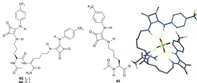
Fig. 16 Molecular structures of dipeptides 43–45 featuring squaramide functionalized side chains and the modelled structure of the adduct [ 43 (SO 4 ) 2- ] 2- showing the possible H-bond patterns responsible for the high binding affinity of 43 towards SO 4 2- in very competitive solvent mixtures. Reproduced with permission from ref. 43. Copyright Wiley 2014.
