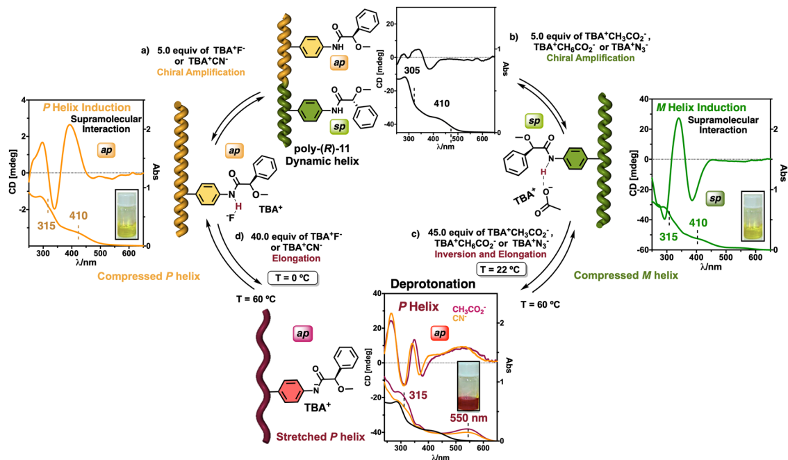
Fig. 23 (a) P and (b) M helix induction in poly-( R )- 11 by addition of 5.0 equiv. of TBA (A = fluoride or cyanide) or (A = acetate, benzoate or azide) respectively. Elongation and P helix induction in poly-( R )- 11 by addition of (c) 45.0 equiv. of TBA (A = acetate, benzoate or azide) at rt or (d) 40.0 equiv. of TBA (A = fluoride or cyanide) at 0 °C. Reproduced from ref. 189 with permission from Elsevier, copyright 2021.
