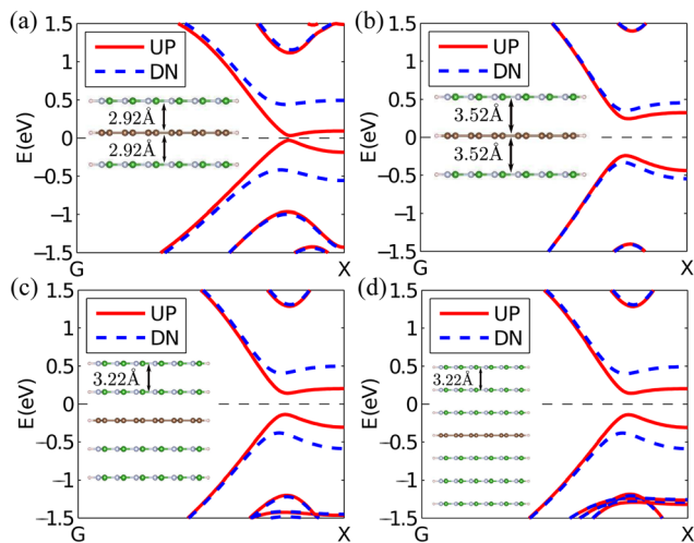
Fig. 5 The band structure for the cases where: (a) the layer distance is decreased by 0.30 \text{ \AA} ; (b) the layer distance is increased by 0.30 \text{ \AA} ; (c) bilayer h-BN nanoribbons distributed on both sides of graphene nanoribbons for the van der Waals heterostructure leads; (d) trilayer h-BN nanoribbons distributed on both sides of graphene nanoribbons for the van der Waals heterostructure leads.
