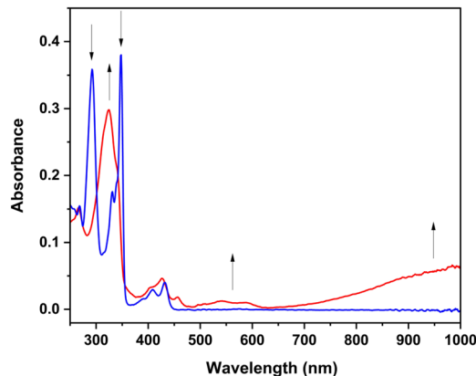
Fig. 9 UV-Vis absorption spectral changes resulting from oxidation of m -ICz-Br (blue) to [ m -ICz-Br] + (red.). Conditions: in CH 2 Cl 2 /Bu 4 NPF 6 at T = 298 K; Pt minigrind in an OTTLE cell.
