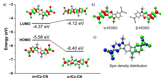
Fig. 3 (a) DFT-calculated (M06-2X/6-31G**) molecular orbital diagram of m -ICz-CN and p -ICz-CN. (b) Calculated highest-occupied single orbitals (HOSO) of α and β electrons for m -ICz-CN. (c) Spin density distribution in the diradical singlet ground state of m -ICz-CN at the (U)M06-2X/6-31G** level of theory with an isosurface value of 0.03 a.u. The blue and green surfaces represent α and β spin densities, respectively.
