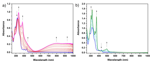
Fig. 10 UV-Vis absorption spectral changes resulting from (a) oxidation of ( m -ICz-CN) 2 (blue) to [ m -ICz-CN] + (purple), and (b) single-step reduction of ( m -ICz-CN) 2 (blue) to [ m -ICz-CN] 2- (green). Conditions: in CH 2 Cl 2 /Bu 4 NPF 6 at T = 298 K; Pt minigrind in an OTTLE cell.
