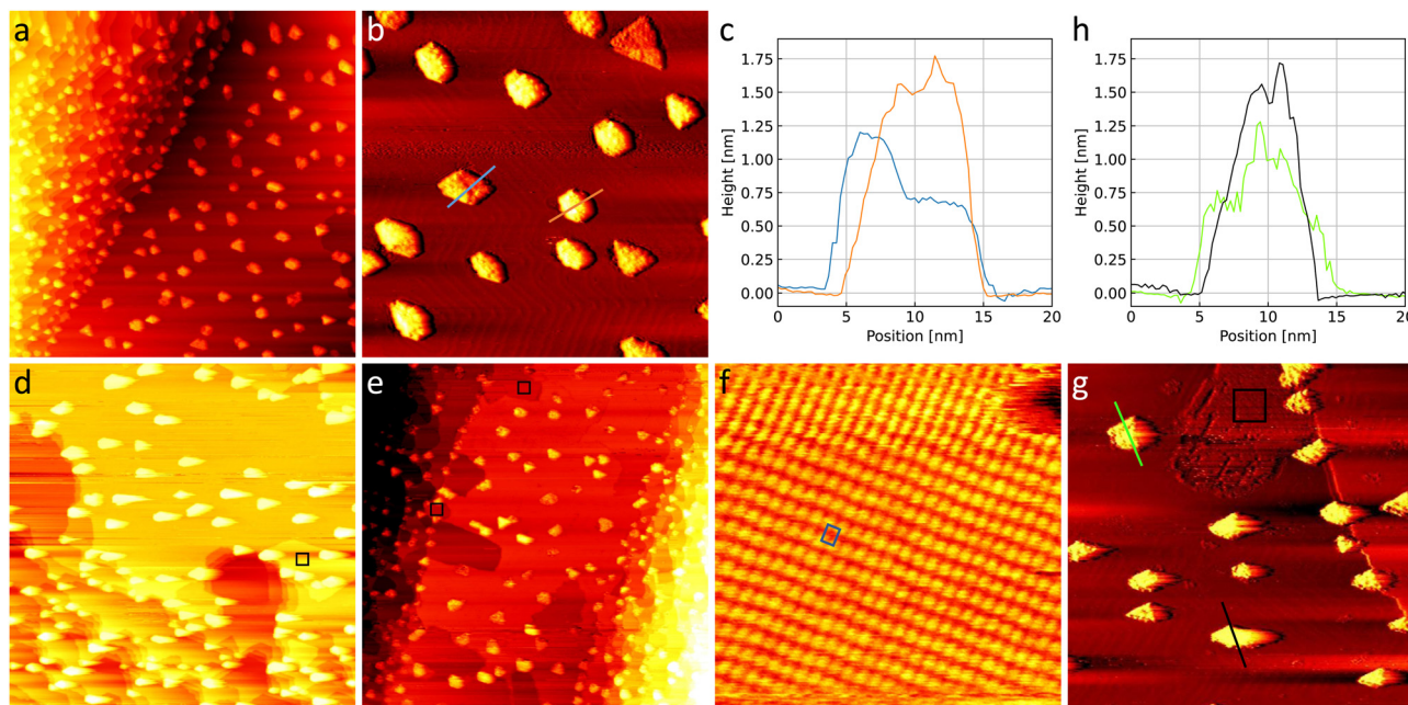
Fig. 5 (a) 300 nm \times 300 nm and (b) 110 nm \times 110 nm STM images of the as-prepared TiO 2 /Au(111) with (c) corresponding height profiles. (d) 300 nm \times 300 nm STM image of TiO 2 /Au(111) after 1 h in 0.8 bar O 2 and (e) 1 h in 1 bar 4O 2 + 1CO, respectively. (f) Representative area of a 10 nm \times 10 nm black square showing the gold oxide unit cell in blue. (g) 110 nm \times 110 nm STM image of a detail of the surface in (d) with corresponding height profiles in (h). In order for the particles and the herringbone reconstruction to be visible simultaneously the images in (b) and (g) were flattened and merged with their derivative in a ratio of 1 : 2 whereas the corresponding profiles in (c) and (h) are taken from the images themselves. Note that the gold oxide island marked with the black square in (g) appears darker in some areas due to an interaction of the STM tip with the titania particles after the gas exposure (details see ESI†). All images are taken in UHV at room temperature with +3 V and 50 pA.
