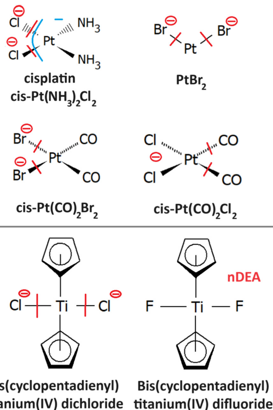
Fig. 10 Radiosensitizers from the group of organometallics and model compounds, whose reactivity with LEEs is discussed in the text: cisplatin (4.1), PtBr 2 (4.2); PtBr 2 (CO) 2 (4.3); titanocenes (4.4). The red line marks the bond broken in the most intense DEA reaction of the molecule identified for the isolated molecule, and the blue line the dissociation for a solvated molecule. The minus sign marks the anionic DEA fragment.
