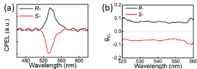
Fig. 39 (a) CPEL spectra and (b) and g_{EL} of spin-LEDs based on (R-NPB)_2(FA_{0.85}Cs_{0.15})_2Pb_3Br_{10} . Reprinted with permission from ref. 51 Copyright©2024 American Chemical Society.
