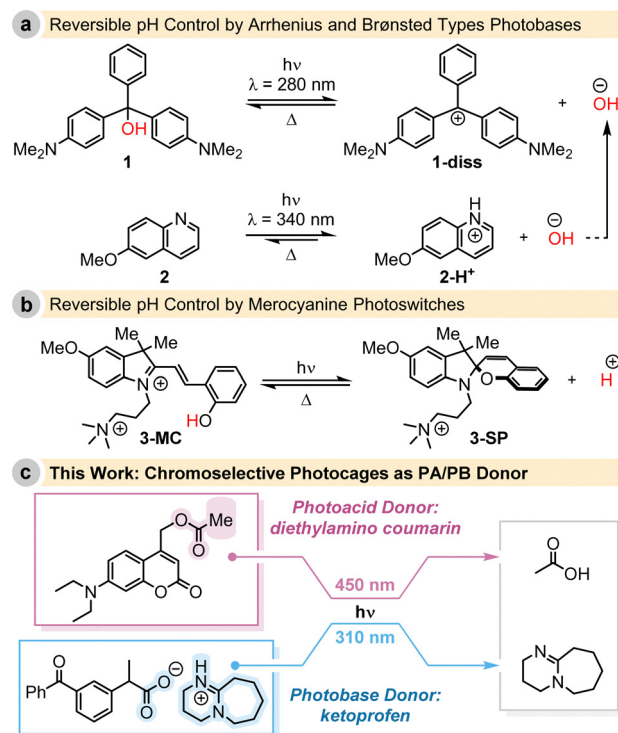
Fig. 1 (a) Reversible pH control by Arrhenius and Brønsted types photobase generator; (b) reversible pH control by Merocyanine photoswitches; (c) our approach: chromosomelective pH regulation by photocages as photoacid/photobase donors.
