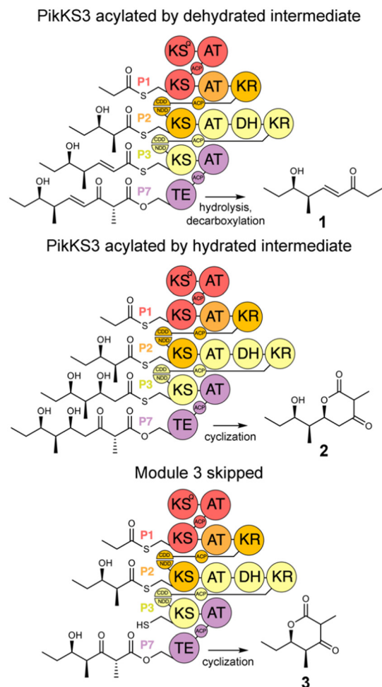
Fig. 2 Polyketide production by P1-P2-P3-P7 and variants. P1-P2-P3-P7, engineered from the updated modules of the pikromycin synthase, synthesizes a β-ketoacid that spontaneously decarboxylates to the tetraketide olefin 1 . Tetraketide lactone 2 is generated when PikKS3 is acylated by the hydrated intermediate. Triketide lactone 3 is generated when the third module, P3, is skipped.
