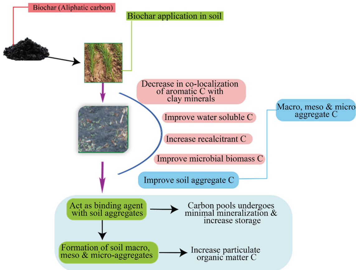
Fig. 2 Possible mechanism of carbon sequestration by biochar inside the soil.
