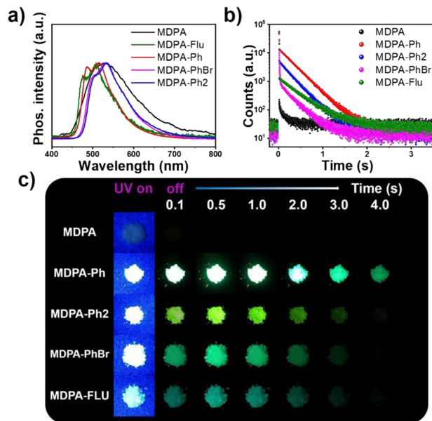
Fig. 2 (a) The RTP spectra of DMAP doping systems with different guests. (b) Phosphorescence intensity decay curves of DMAP doping systems with different guests. (c) Photographs of DMAP doping systems with different guests, photographs were taken under a 365 nm UV lamp (on or off), and the times after the UV lamp was turned off are also given in the inset.
