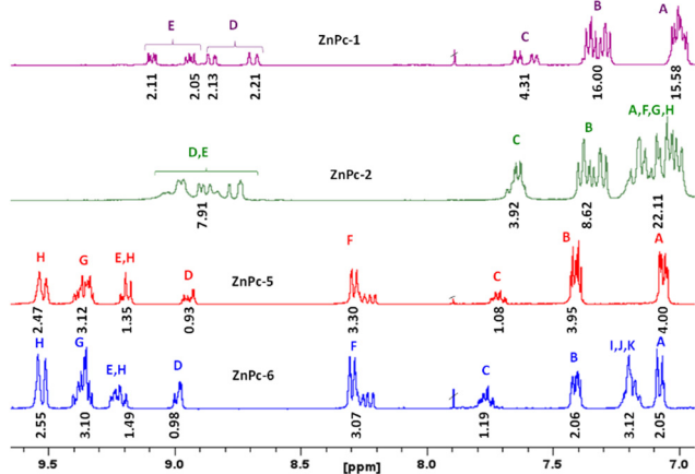
Fig. 3 1 H-NMR spectra of ZnPcs in THF- d 8 .
