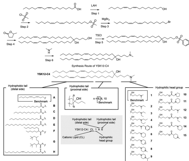
Fig. 4 The synthesis route and structure of pH-sensitive cationic lipid YSK12-C4 . Magnesium bromide ( MgBr_2 ), 4-toluenesulfonyl chloride (TfCl).
