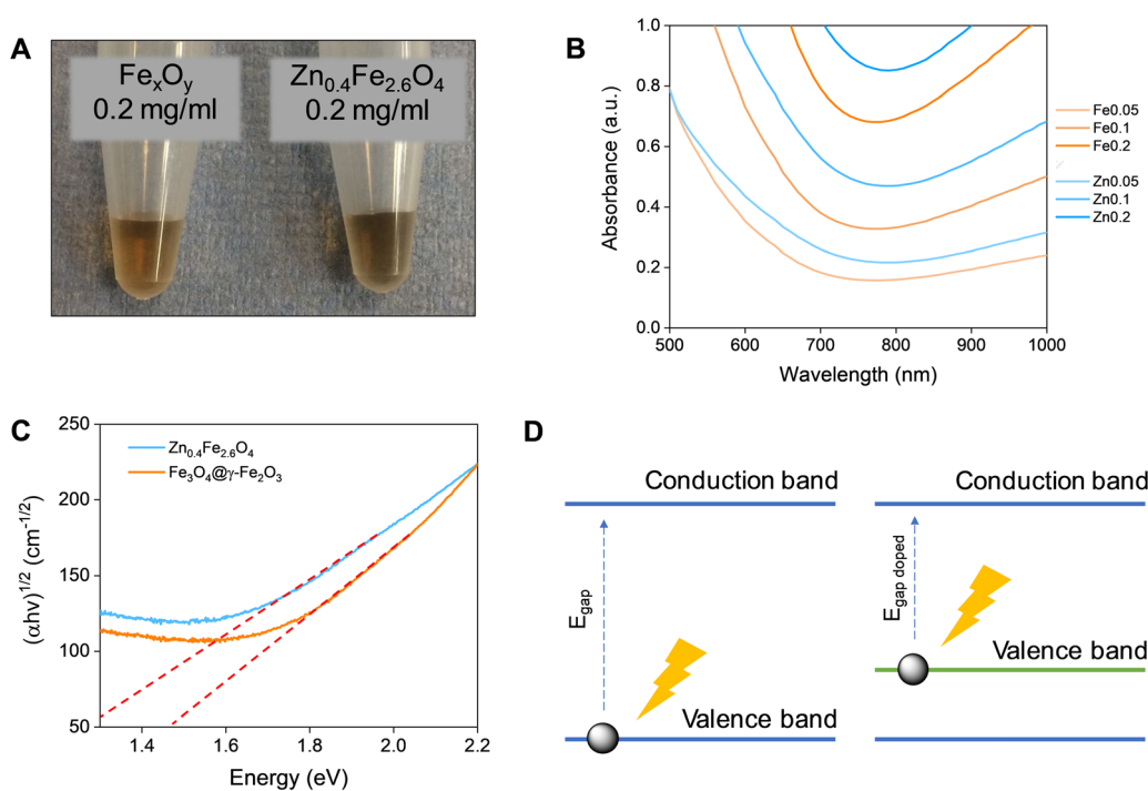
Fig. 5 (A) Digital photographs of \text{Fe}_3\text{O}_4@ \gamma\text{-Fe}_2\text{O}_3 (left) and \text{Zn}_{0.4}\text{Fe}_{2.6}\text{O}_4 (right) NPs at a concentration of 0.2 \text{ mg}_{\text{Fe+Zn}} \text{ ml}^{-1} . (B) UV-Vis-NIR spectra of \text{Fe}_3\text{O}_4@ \gamma\text{-Fe}_2\text{O}_3 and \text{Zn}_{0.4}\text{Fe}_{2.6}\text{O}_4 NPs for concentrations between 0.05\text{--}0.2 \text{ mg}_{\text{Fe or Zn}} \text{ ml}^{-1} . (C) Tauc plots of \text{Fe}_3\text{O}_4@ \gamma\text{-Fe}_2\text{O}_3 and \text{Zn}_{0.4}\text{Fe}_{2.6}\text{O}_4 NPs with extrapolation of the linear region to y = 0 . (D) A scheme of bandgap decrease by doping.
