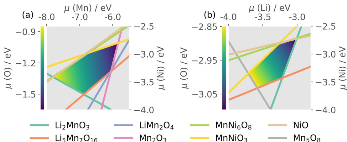
Fig. 3 The chemical potential space of P_{4/32}LiMn_{1.5}Ni_{0.5}O_4 , (a) where chemical potential of Li was set to an average value of -3.35 eV; (b) where chemical potential of Mn was set to an average value of -6.42 eV. Yellow/dark-blue colour shadings represent p/n-type conditions.
