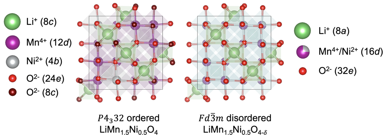
Fig. 1 Representative structures (with Wyckoff positions) of the P4_32 ordered and Fd\bar{3}m disordered LMNO.
