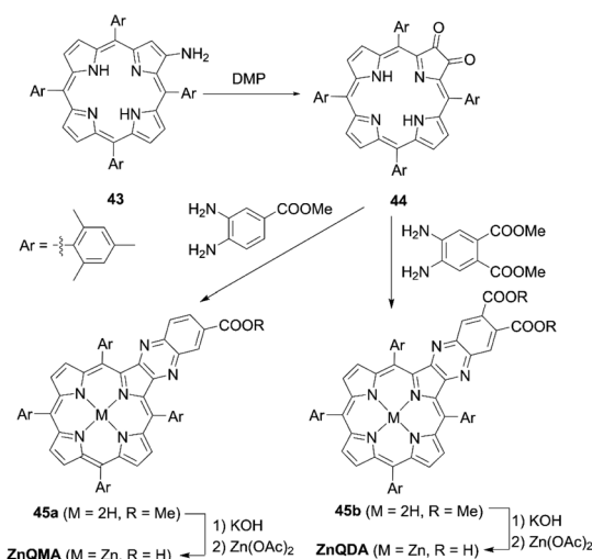
Scheme 8 Syntheses of ZnQMA and ZnQDA .
