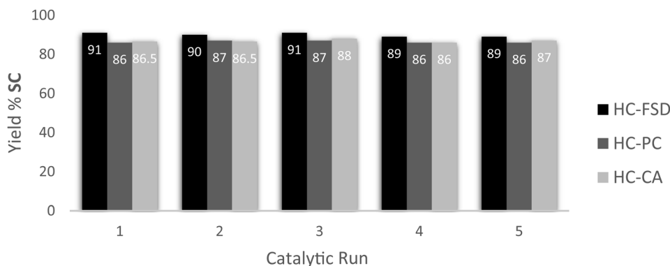
Fig. 9 Recycling catalytic test for the coupling of SO and CO 2 catalyzed by HC-FSD, HC-PC and HC-CA. Reaction conditions: 0.875 mmol SO (100 \mu L), autoclave, p (CO 2 ) 3 bar, catalyst loading 10 wt%, temperature 70 ^{\circ} C, 7 h. Isolated yields are given, after purification of the reaction crude by flash column chromatography. Yield of SC was the average after two runs. Selectivity was > 99% for all catalytic runs.
