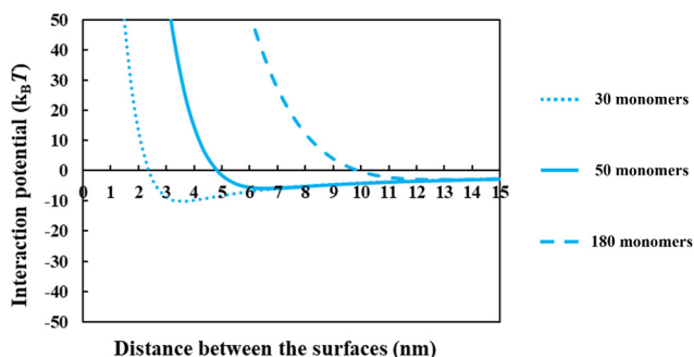
Fig. 9 The interaction potential plotted against the separation distance between a pair of droplets, induced by the adsorbed protein + maltodextrin conjugates consisting of soy protein fragment \text{Asn}^{356}\text{-Arg}^{425} with attached hydrophilic chains of various sizes ( i.e. 30, 50 and 180 monomers). Droplets are assumed to be 1\ \mu\text{m} in diameter. All the results were calculated with a background electrolyte volume fraction of 0.01 (roughly equating to 100 mM NaCl) and at a solution pH = 5.5.
