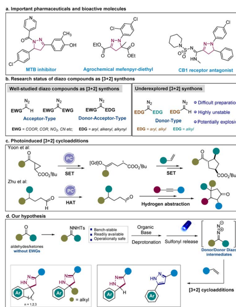
Scheme 1 Visible-light mediated [3 + 2] cycloadditions and our design.
