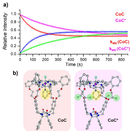
Fig. 6 (a) Relative time evolution of [\text{CoC}(\text{Py})_{\text{IN}}]^+ (red), [\text{CoC}(\text{Py}^-)]^+ (blue), [\text{CoC}^*(\text{Py})_{\text{IN}}]^+ (magenta), and [\text{CoC}^*(\text{Py}^-)]^+ (green) in a single DRL experiment carried out at 40 °C in \text{CHCl}_3 with 200 equiv. pyridine and 200 equiv. pyridine-D5. Dots are experimental data points, and lines correspond to fittings of experimental data by eqn (S1) and (S2).† (b) DFT-calculated structures of ^1[\text{CoC}(\text{Cl}_{\text{OUT}})(\text{Py}_{\text{IN}})] and ^1[\text{CoC}^*(\text{Cl}_{\text{OUT}})(\text{Py}_{\text{IN}})] optimized with B3LYP-D3/def2svp.
