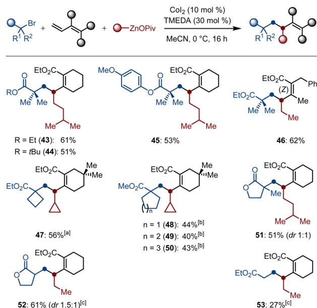
Scheme 4 Substrate scope for the cobalt-catalyzed selective 1,2-dialkylation of dienoates. Reaction conditions: alkyl bromides (0.15 mmol, 1.0 equiv.), dienoates (1.5 equiv.), Alk-ZnOPiv (2.5 equiv.), \text{Co}_2 (10 mol%), TMEDA (30 mol%), MeCN (1.5 mL), 0 °C, 16 h. [a] 3 mmol scale. [b] Dienoates (0.15 mmol, 1.0 equiv.), alkyl bromides (2.0 equiv.), Alk-ZnOPiv (2.5 equiv.), \text{Co}_2 (10 mol%), MeCN (1.5 mL), 0 °C, 16 h. [c] w/o TMEDA, at 25 °C.
