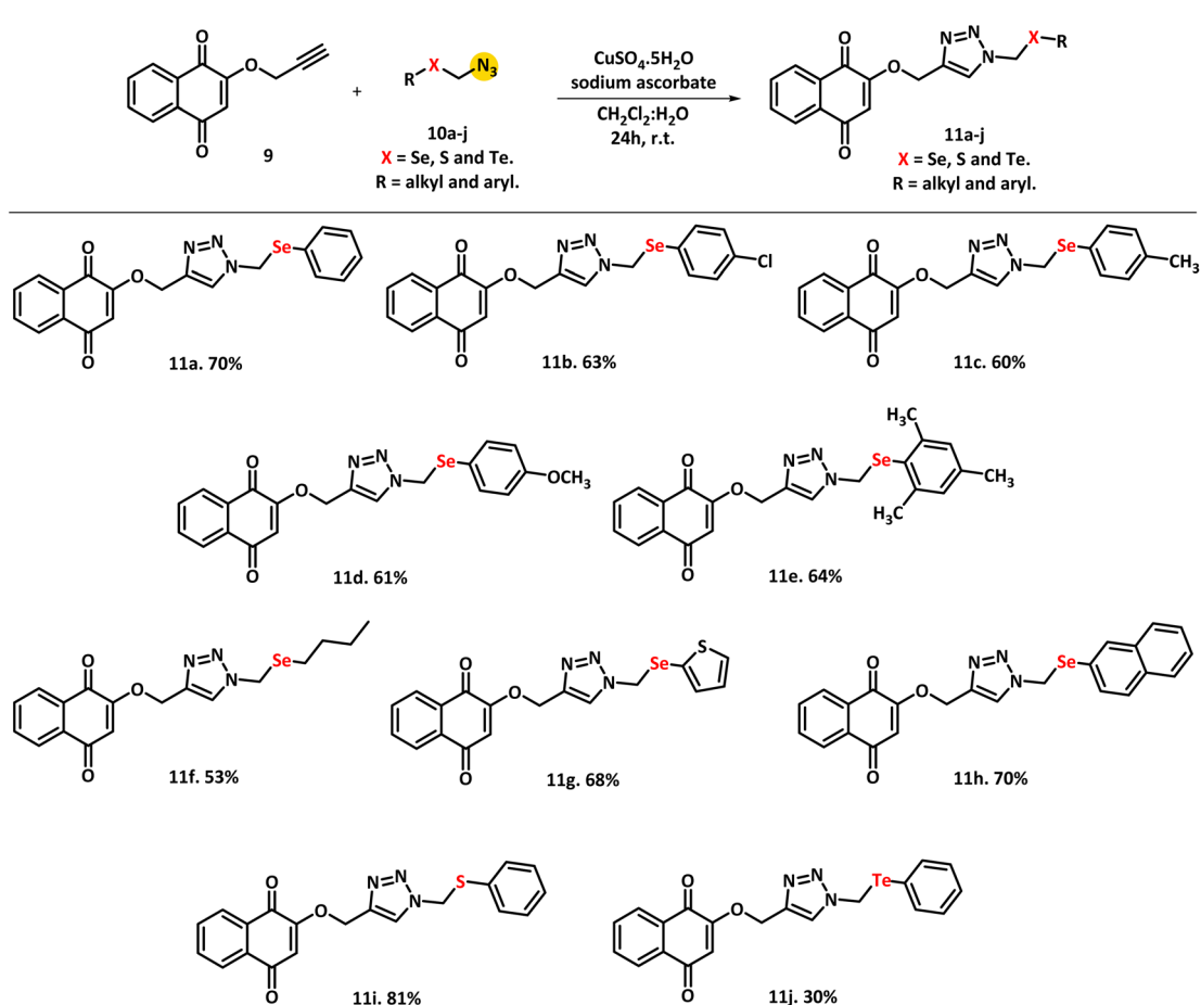
Scheme 4 Synthesis of chalcogen-naphthoquinone-1,2,3-triazoles 11a–j.
