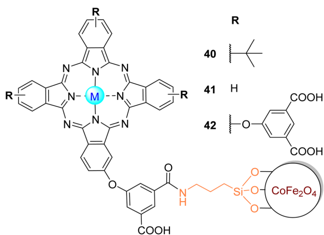
Fig. 12 Zn40–Zn42 coupled to \text{CoFe}_2\text{O}_4 MNP used by Nyokong and co-workers 142,143 for the degradation of MO.
