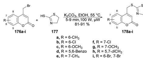
Scheme 63 Synthesis of coumarin–thiazoline hybrids 178a–i .
