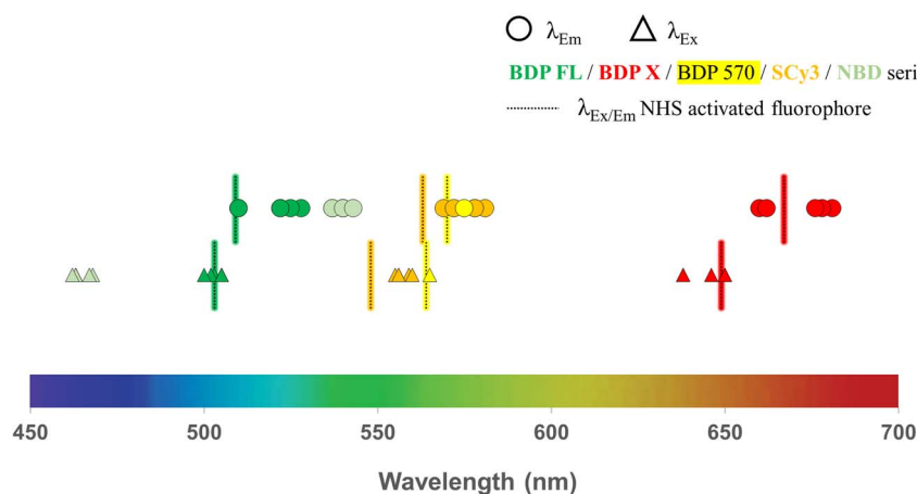
Fig. 2 Fluorescence characteristics (excitation and emission wavelengths) determined from spectra recorded in ethanol solutions for all new P-gp targeted fluorescent conjugates and commercial NHS-activated fluorophores (BDP FL, BDP X, BDP 570 and SCy3 series).
