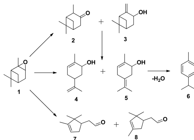
Scheme 17 Products of isomerisation of \alpha -pinene oxide; (1) \alpha -pinene oxide, (2) isopinocampone, (3) pinocarveol, (4) trans -carveol, (5) 2-methyl-5-(propan-2-ylidene)cyclohex-2-enol, (6) p -cymene, (7) campholenic aldehyde and (8) fencholenic aldehydes. 10
