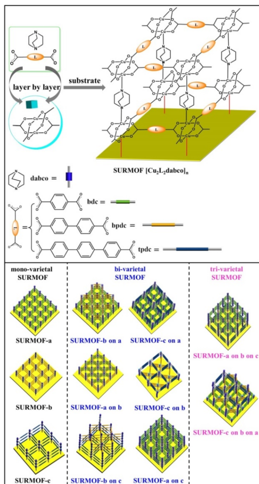
Scheme 1 Schematic illustration for the preparation of mono-varietal SURMOFs [\text{Cu}_2\text{L}_2\text{dabco}]_n ( L = \text{bdc}, \text{bpdc}, \text{and tpdc} ) and their multiple (bi-varietal and tri-varietal) SURMOFs on substrate surfaces by using a LPE layer by layer method.
