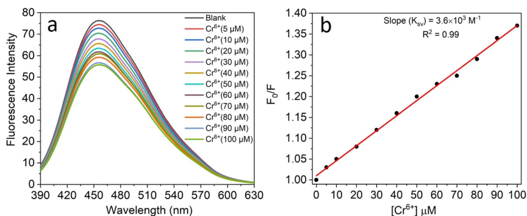
Fig. 4 (a) Fluorescence spectra of CNPs (2.0 mg mL ^{-1} ) in the presence of different amounts of Cr ^{6+} from the top to bottom: 5, 10, 20, 30, 40, 50, 60, 70, 80, 90, and 100 \mu\text{M} in double-distilled water ( \lambda_{\text{exc}} = 370 nm) and (b) plot of F_0/F against the concentration of Cr ^{6+} (Stern–Volmer quenching response) at 454 nm.
