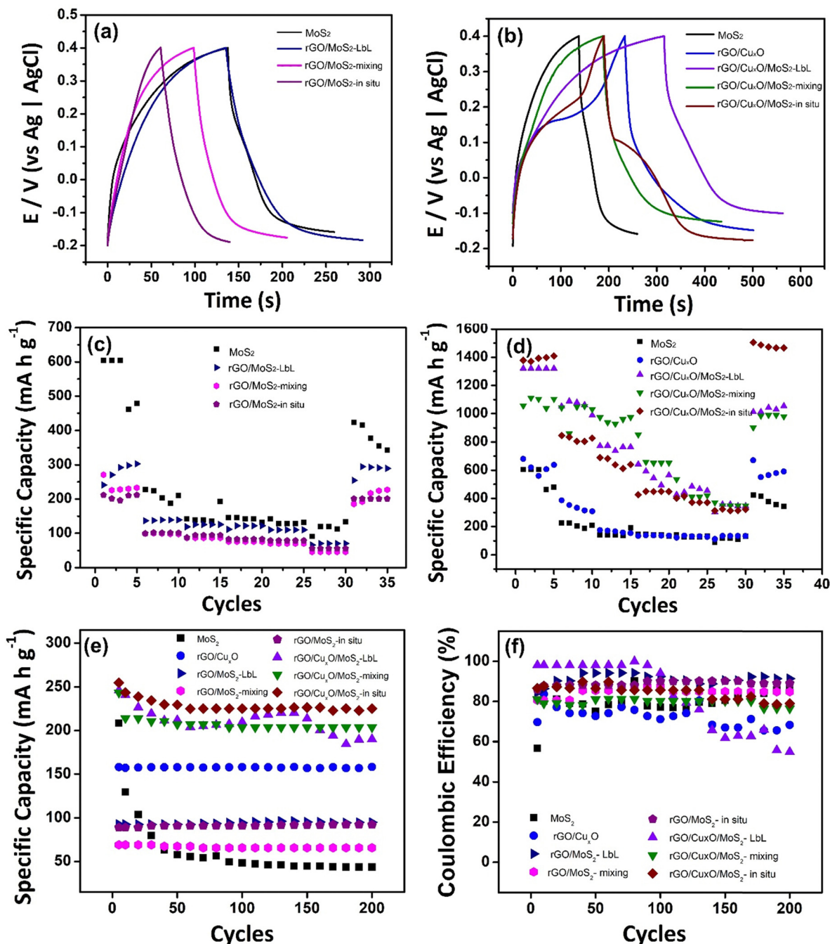
Fig. 8 Charge and discharge curves (a) and (b); specific capacity of the discharge process (c) and (d) at different current densities (0.1, 0.25, 0.5, 0.75, 1 and 2 \text{ A g}^{-1} ); specific capacity measured during 200 cycles at 2 \text{ A g}^{-1} (e) and Coulombic efficiency (f) of the nanocomposites in 0.1 \text{ mol L}^{-1} NaCl aqueous solution and the potential range of -0.2 to 0.4 \text{ V} .
