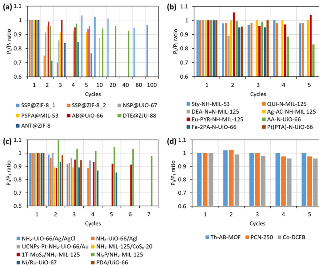
Fig. 3 Photo-switching fatigue of (a) guest@MOF systems, (b) post-synthetically modified NH 2 -MOFs, (c) MOF composites, and (d) MOFs containing photo-responsive ligands. Performance at cycle i divided by performance at cycle 1 ( P_i/P_1 ratio). The parameters used to evaluate the performance at each cycle are: proton conductivity on/off ratio (SSP@ZIF-8_1), Li + conductivity (SSP@ZIF-8_2), electrical conductivity (NSP@UiO-67), NaCl adsorption loading (PSPA@MIL-53), ion flux (AB@UiO-66), emission intensity at 613 nm (DTE@ZJU-88), enhancement factor (ANT@ZIF-8), photo-controllable cargo release (Sty-NH-MIL-53), benzyl alcohol oxidation (QUI-N-MIL-125), benzaldehyde production (DEA-N=N-MIL-125), MB degradation (Ag-AC-NH-MIL-125), catalytic conversion (Eu-PYR-NH-MIL-125), AO7 degradation (AA-N-UiO-66), \alpha -acyloxy amide yield (Fe-2PA-N-UiO-66), HER rate (Pt(PTA)-N-UiO-66), RhB photodegradation (NH 2 -UiO-66/Ag/AgCl), TC photodegradation (NH 2 -UiO-66/AgI), H 2 generation (UCNP-Pt-NH 2 -UiO-66/Au), RhB photodegradation (NH 2 -MIL-125/CoS x -20), H 2 generation (1T-MoS 2 /NH 2 -MIL-125), H 2 generation (Ni 2 P/NH 2 -MIL-125), CO catalytic turnover number (Ni/Ru-UiO-67), MB conversion (PDA/UiO-66), cis -isomer fraction (Th-AB-MOF), CO 2 uptake (PCN-250), and 5-aryl-2-imino-1,3-oxathiolane yield (Co-DCFB) [data adapted from ref. 41–44,47–49,86–104].
