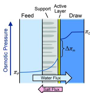
Fig. 11 Illustration of the semipermeable membrane cross section composed of an active layer and a support layer. A qualitative presentation of osmotic pressure profile across the membrane is presented (figures and captions reproduced from with permission ref. 78 with permission from Royal Society of Chemistry, copyright 2016).
