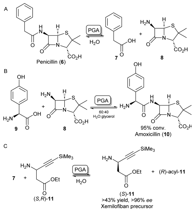
Scheme 3 Applications of penicillin G acylase (PGA). (A) PGA catalyses the hydrolysis of penicillin into 7 and 8. (B) PGA can reinstall alternative acyl side chains such as 9 to synthesize analogous antibiotics like amoxicillin 10. 26 (C) Racemic \beta -aminoester 11 can be deracemized on an industrial scale to obtain drug precursor (S)-11 in high ee's. 34
