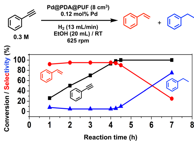
Fig. 5 Hydrogenation of phenylacetylene with Pd@PDA@PUF (8 cm 3 ); 0.12 mol% Pd. Reaction conditions: PA (6 mmol), Pd (7 × 10 -3 mmol), EtOH (20 mL), H 2 flow rate (13 mL min -1 ), room temperature, 625 rpm.
