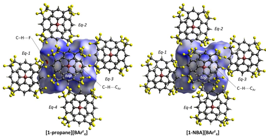
Fig. 3 Hirshfeld surfaces mapped over d_{\text{norm}} for [1\text{-NBA}]^+ and [1\text{-propane}]^+ within the octahedral arrays of neighbouring [\text{BAR}^{\text{F}}_4]^- anions with the anion labelling system indicated. Views are taken from above the 'top' anion looking down the \text{B}_{\text{top}} \cdots \text{Rh} \cdots \text{B}_{\text{bottom}} axis; the 'bottom' anion is obscured by the cation surface.
