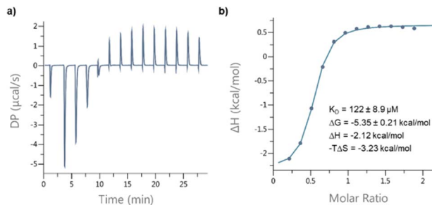
Fig. 7 ITC analysis of the interaction between I and T_1 in CH_3OH : (a) raw data; (b) fitted curve.
