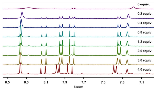
Fig. 8 Stacked ^1H NMR spectra of T_1 ( CD_3OD : D_2O = 9 : 1 ) upon titration of increasing portions of I.
