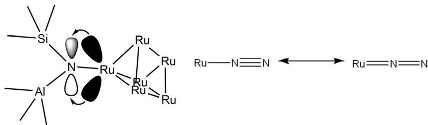
Fig. 17 Schematic (left) of Ru 5d to substituted N 2p back-donation with a Ru 6 N 6 cluster anchored to a bridging N to give electron deficient Ru atoms (only one Ru–N bond pictured, for clarity). Schematic (right) of decreasing Ru–N double bond character due to the electron deficient Ru atoms before the final desorption of Ru-bound molecular N 2 during ammonia decomposition.
