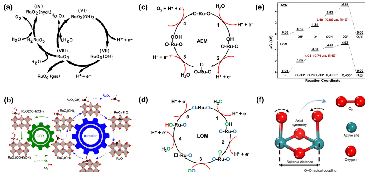
Fig. 4 (a) Model for the oxygen evolution and corrosion on Ru and \text{RuO}_2 electrodes. 85 (b) Schematic representation of the found coupling between corrosion and oxygen evolution reaction for the \text{RuO}_2(110) surface. 87 (c) The adsorbate evolution mechanism (AEM). (d) The lattice oxygen evolution mechanism (LOM). (e) The free energy diagrams of the two mechanisms of LOM and AEM for Co-doped \text{RuO}_2 . 97 (f) O–O radical coupling promoted by symmetric dual active sites. 99
